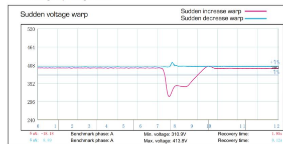
Emergency voltage curve
